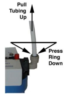
Disconnecting Tubing
